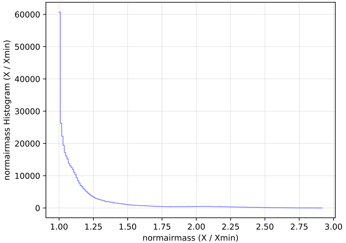
internal_u_expt60_nscale0.9v3.4_10yrs WFD z band: normairmass Histogram
