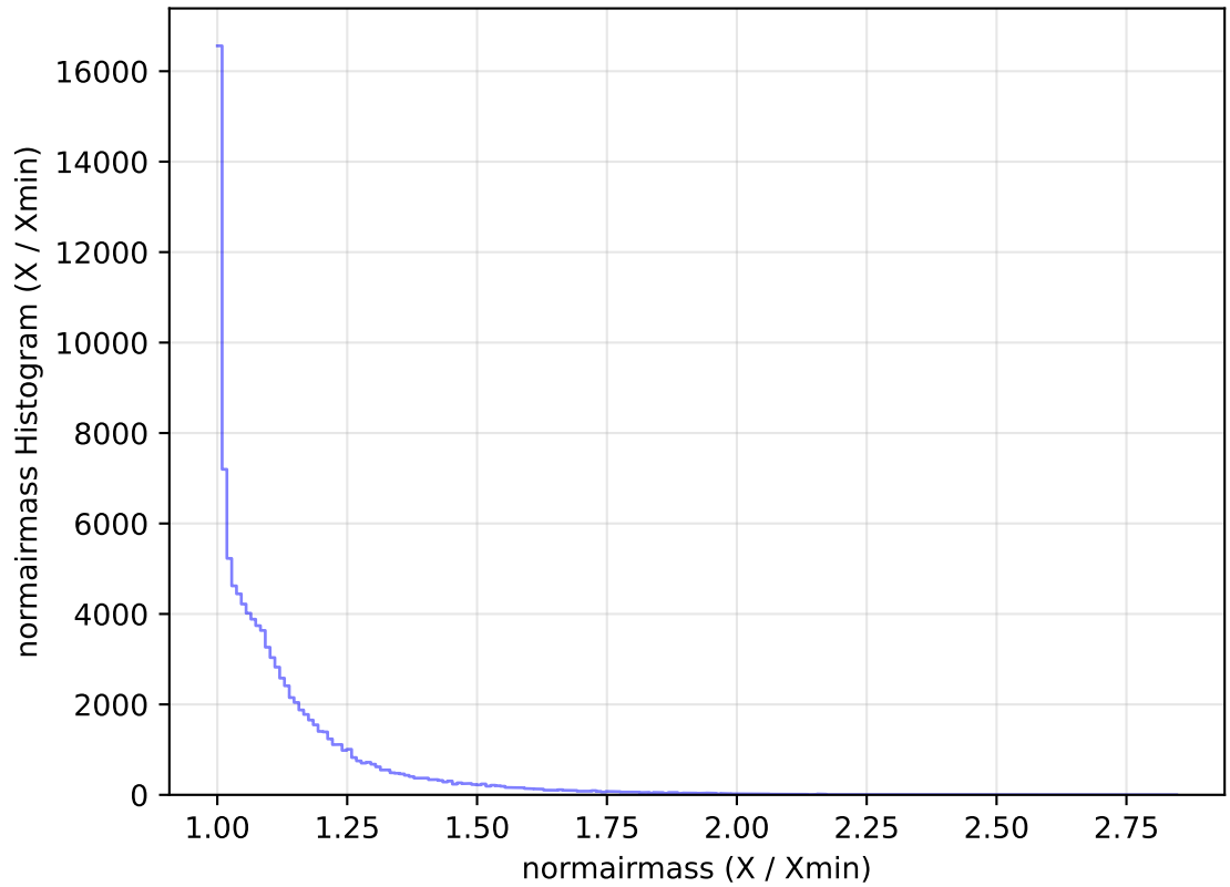
internal_u_expt60_nscale0.9v3.4_10yrs WFD u band: normairmass Histogram
