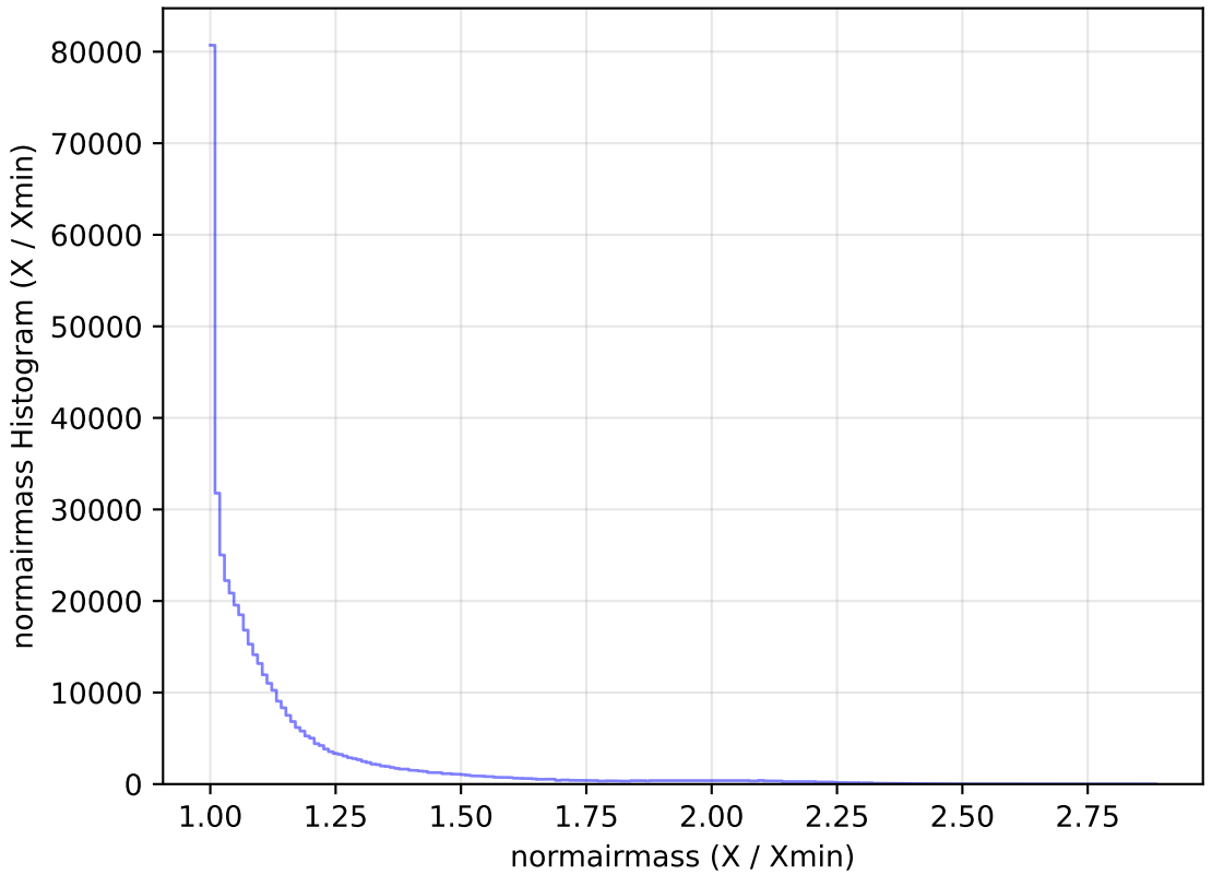
internal_u_expt60_nscale0.9v3.4_10yrs WFD r band: normairmass Histogram
