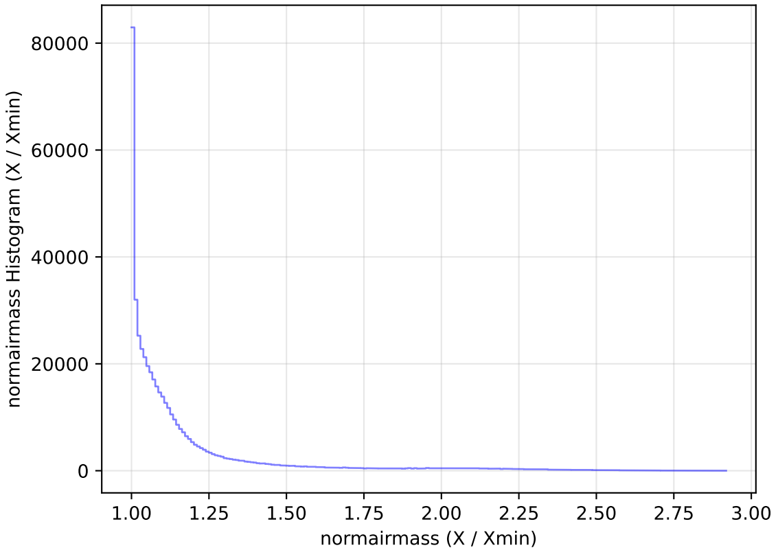
internal_u_expt60_nscale0.9v3.4_10yrs WFD i band: normairmass Histogram
