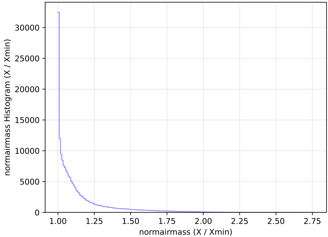
internal_u_expt60_nscale0.9v3.4_10yrs WFD g band: normairmass Histogram
