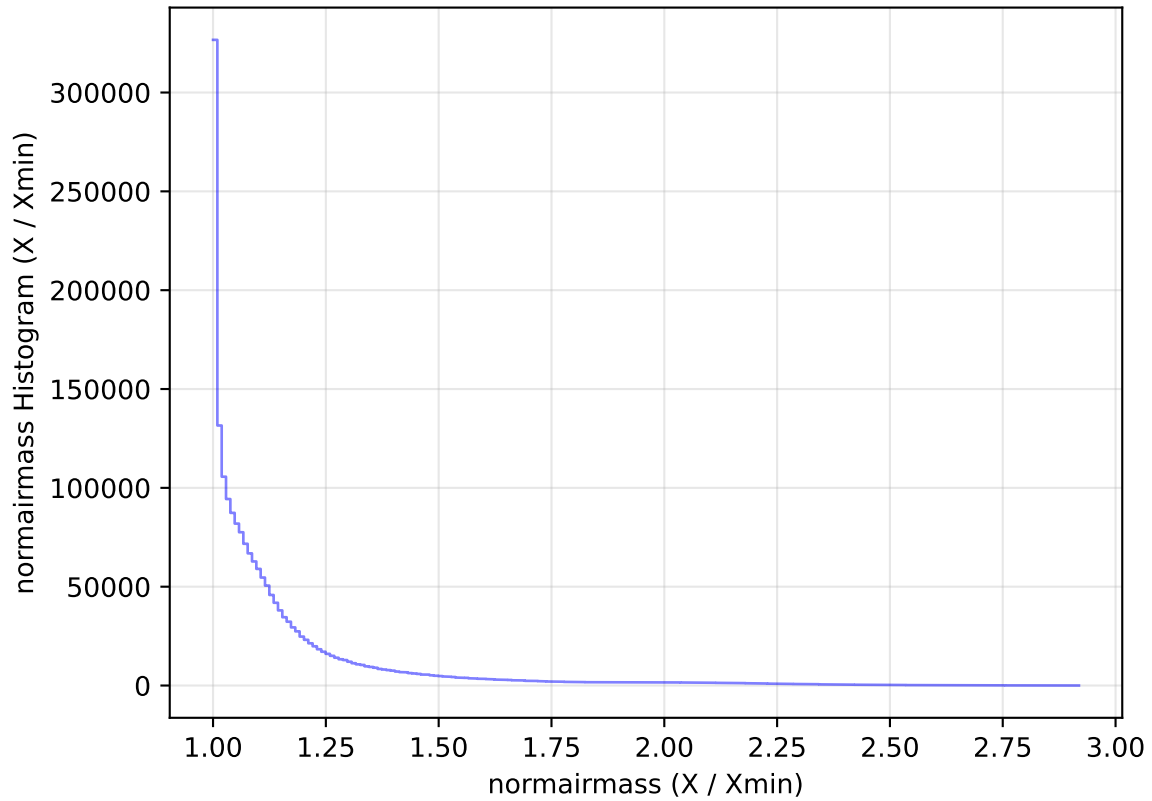
internal_u_expt60_nscale0.9v3.4_10yrs WFD all bands: normairmass Histogram
