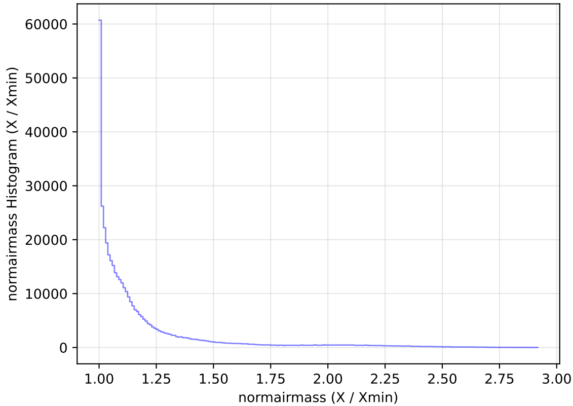
internal_u_expt60_nscale0.9v3.4_10yrs All sky z band: normairmass Histogram
