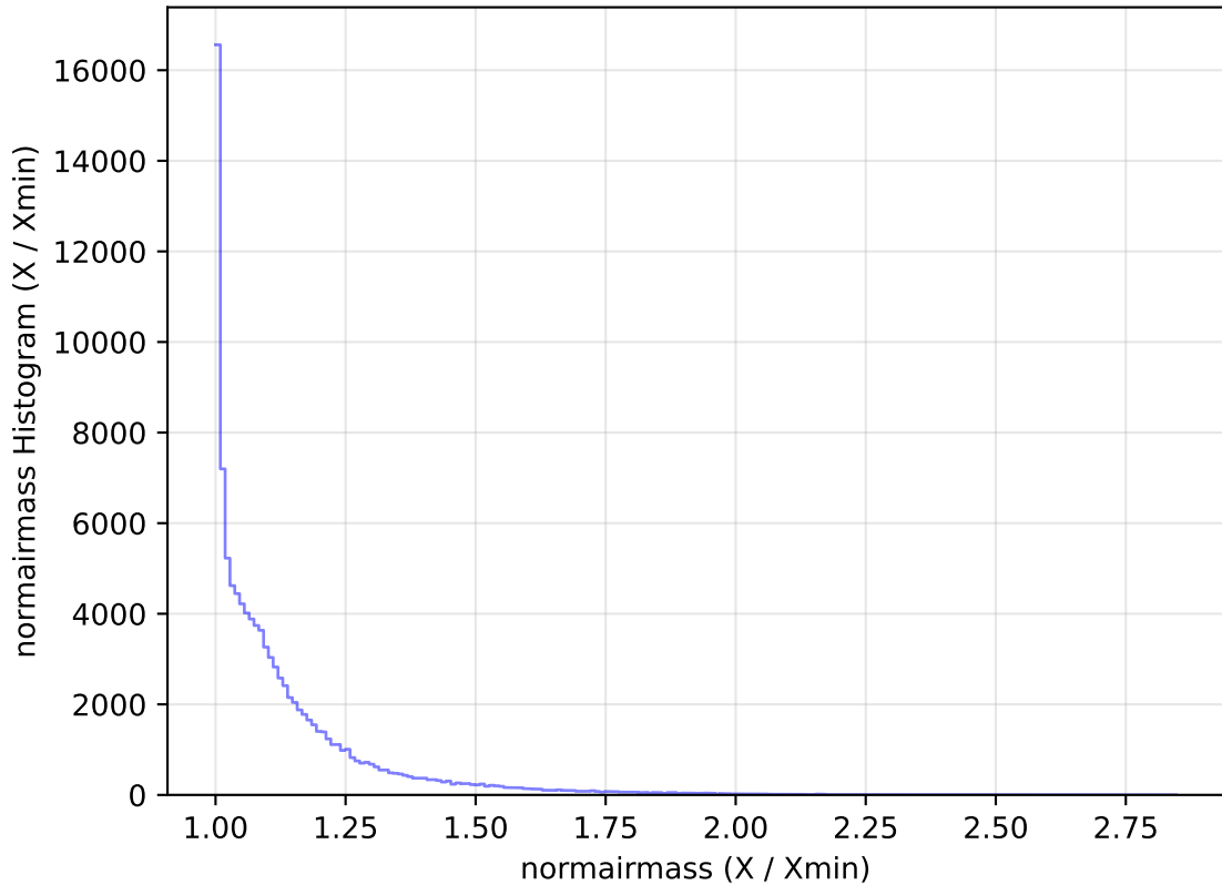
internal_u_expt60_nscale0.9v3.4_10yrs All sky u band: normairmass Histogram
