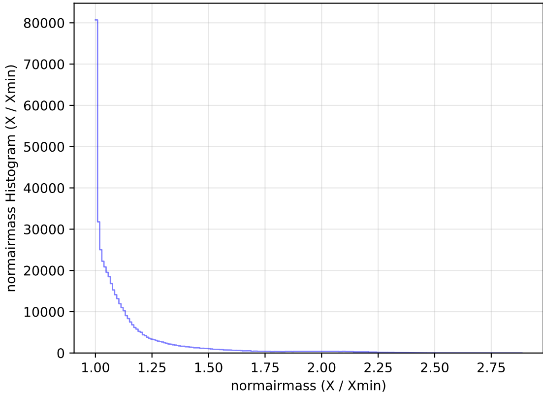
internal_u_expt60_nscale0.9v3.4_10yrs All sky r band: normairmass Histogram
