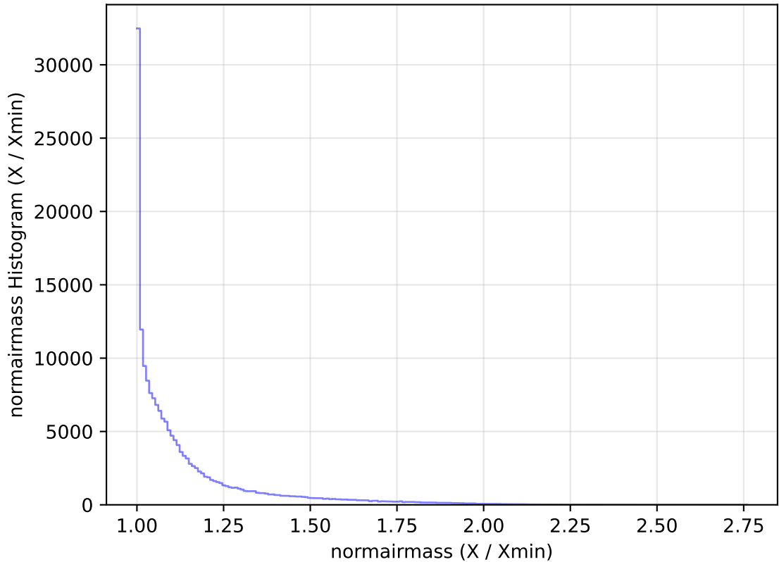
internal_u_expt60_nscale0.9v3.4_10yrs All sky g band: normairmass Histogram
