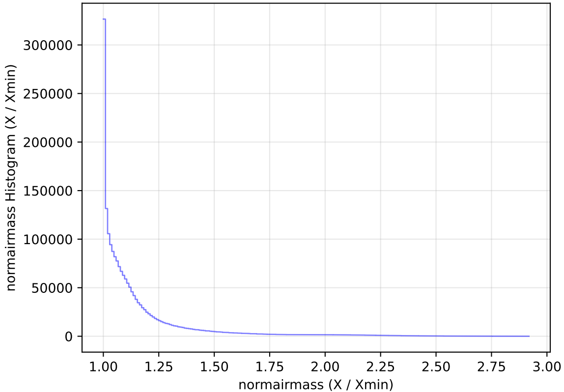
internal_u_expt60_nscale0.9v3.4_10yrs All sky all bands: normairmass Histogram
