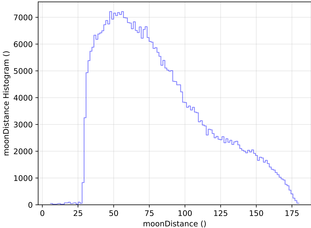
internal_u_expt60_nscale0.9v3.4_10yrs WFD z band: moonDistance Histogram
