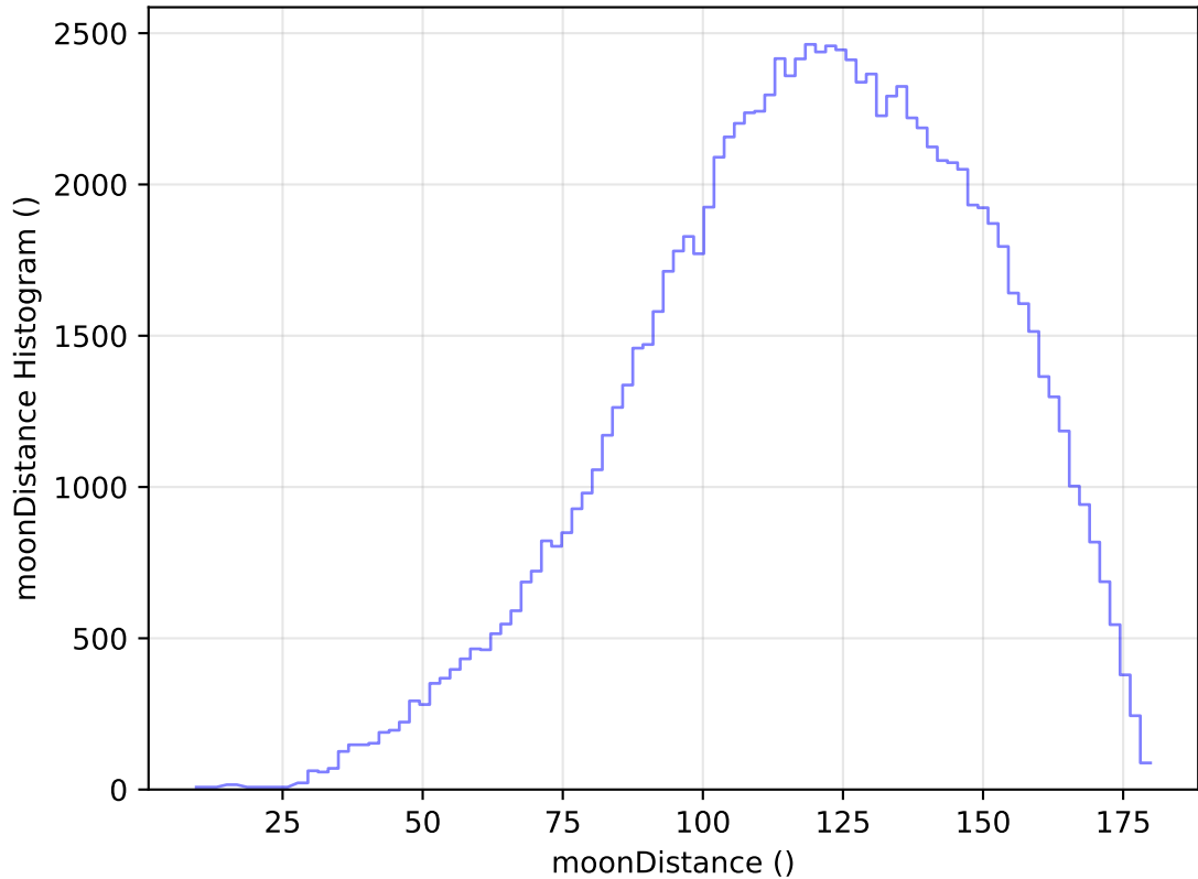
internal_u_expt60_nscale0.9v3.4_10yrs WFD u band: moonDistance Histogram
