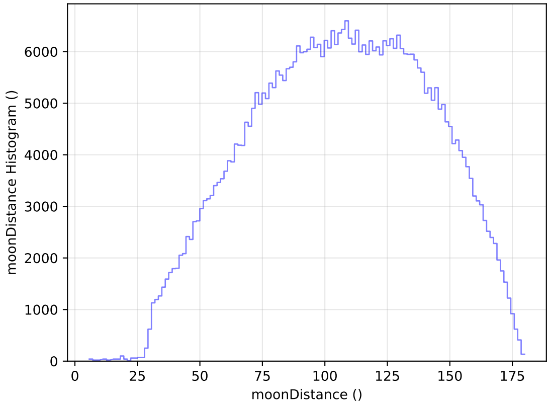
internal_u_expt60_nscale0.9v3.4_10yrs WFD r band: moonDistance Histogram
