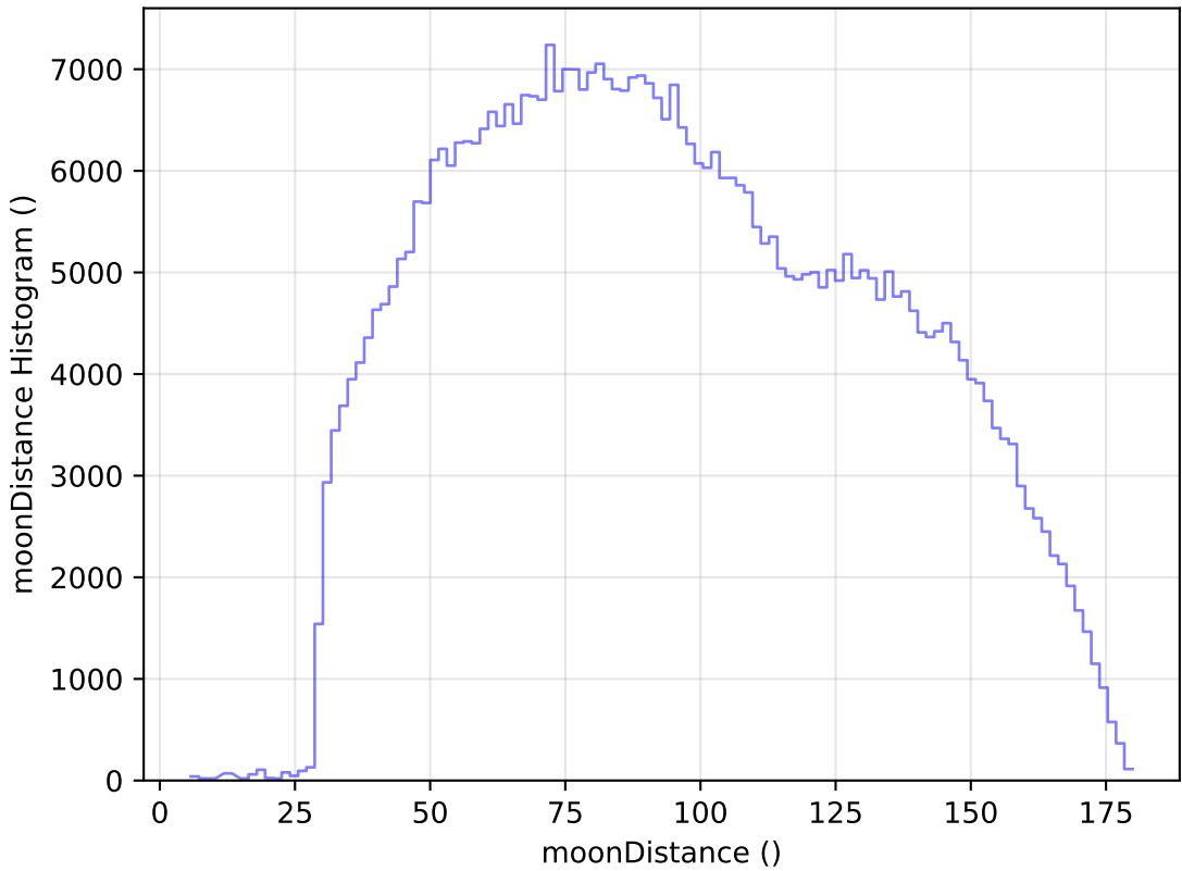
internal_u_expt60_nscale0.9v3.4_10yrs WFD i band: moonDistance Histogram
