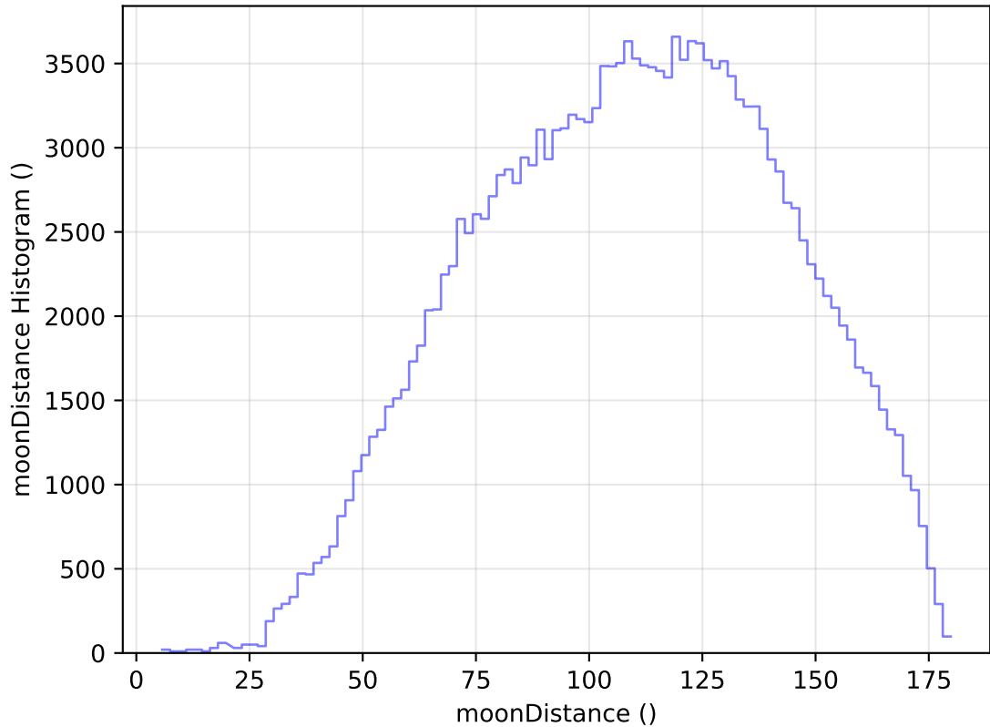
internal_u_expt60_nscale0.9v3.4_10yrs WFD g band: moonDistance Histogram
