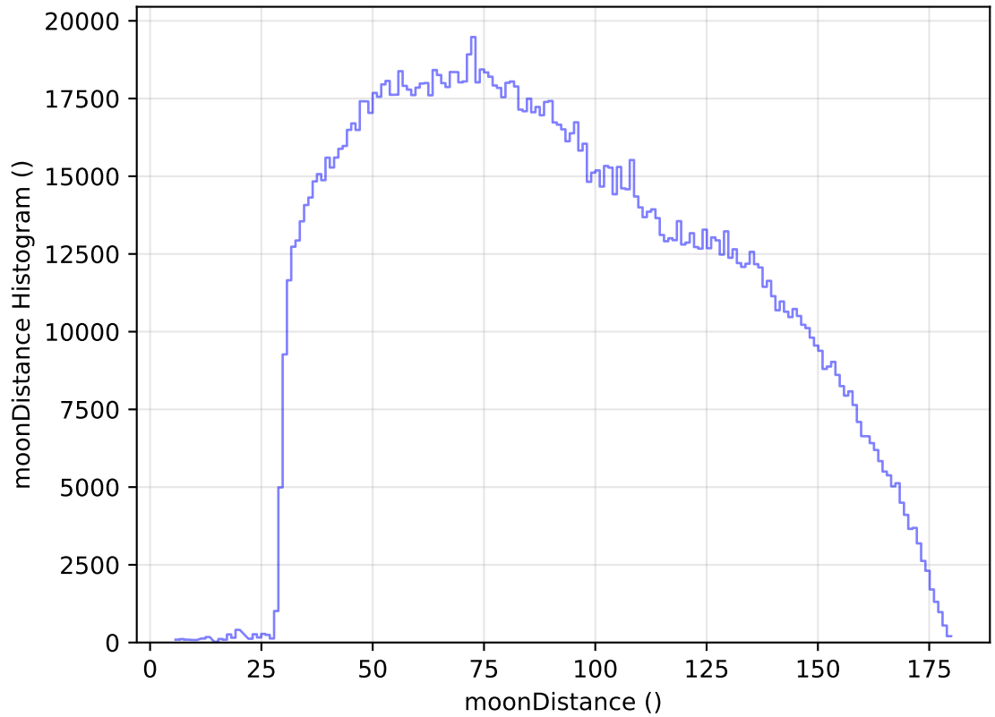
internal_u_expt60_nscale0.9v3.4_10yrs WFD all bands: moonDistance Histogram
