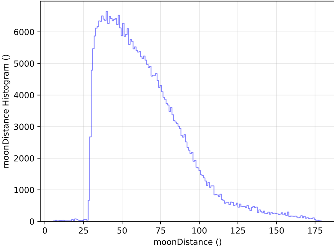
internal_u_expt60_nscale0.9v3.4_10yrs All sky y band: moonDistance Histogram
