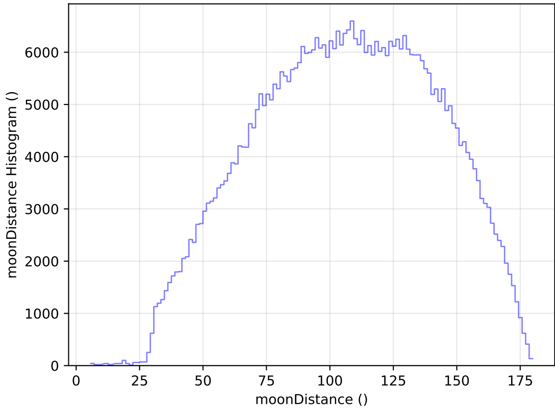
internal_u_expt60_nscale0.9v3.4_10yrs All sky r band: moonDistance Histogram
