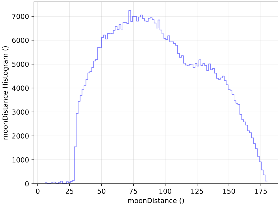
internal_u_expt60_nscale0.9v3.4_10yrs All sky i band: moonDistance Histogram
