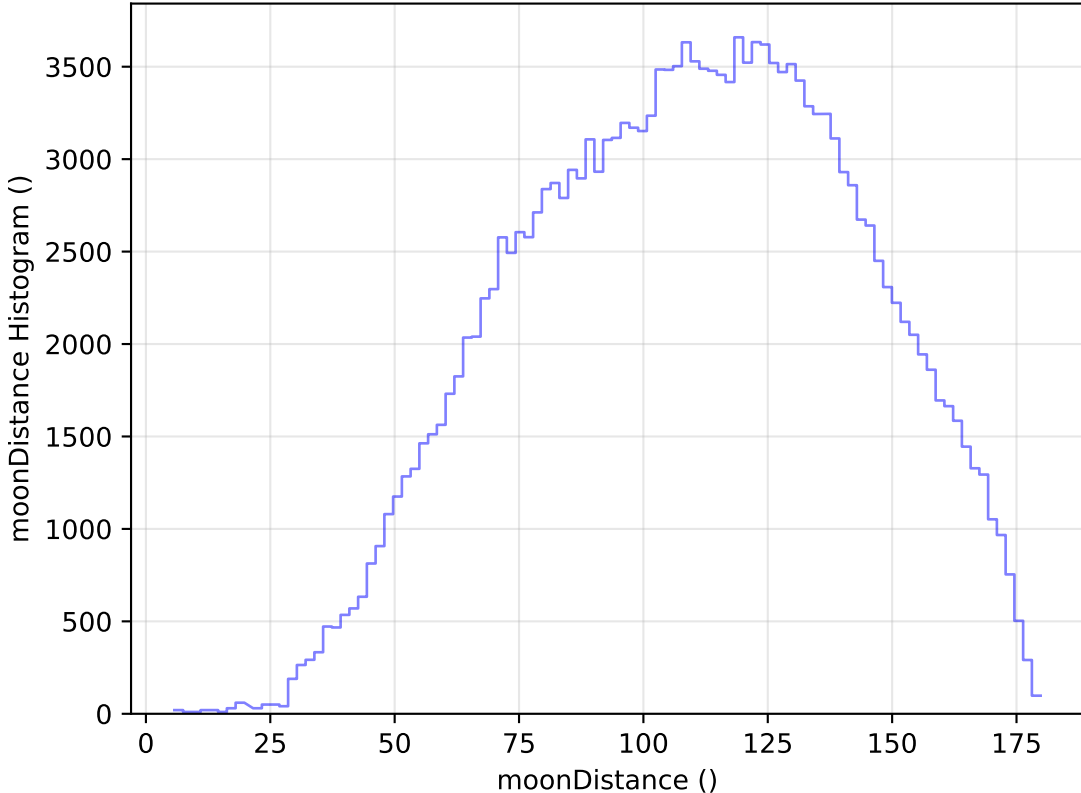
internal_u_expt60_nscale0.9v3.4_10yrs All sky g band: moonDistance Histogram
