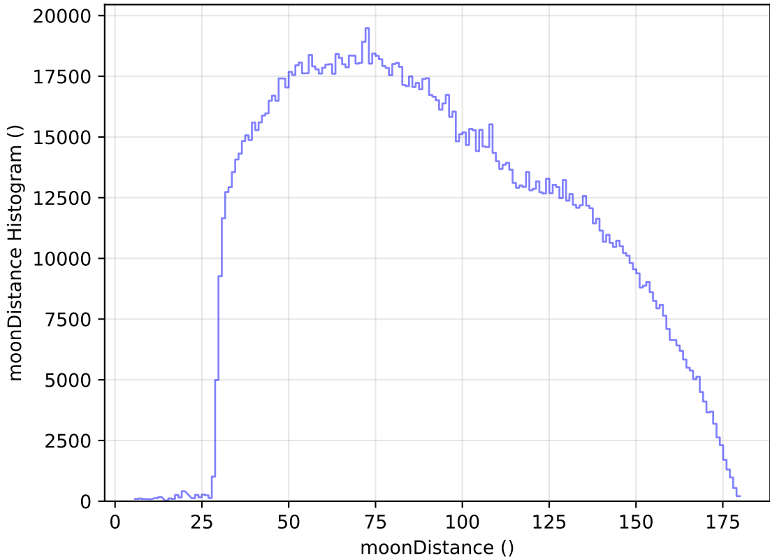
internal_u_expt60_nscale0.9v3.4_10yrs All sky all bands: moonDistance Histogram
