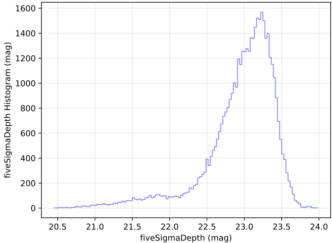
internal_u_expt60_nscale0.9v3.4_10yrs Yr 1 z band: fiveSigmaDepth Histogram
