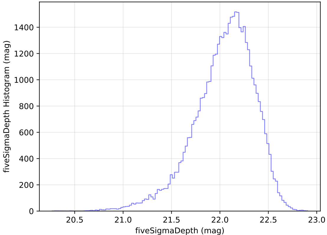
internal_u_expt60_nscale0.9v3.4_10yrs Yr 1 y band: fiveSigmaDepth Histogram
