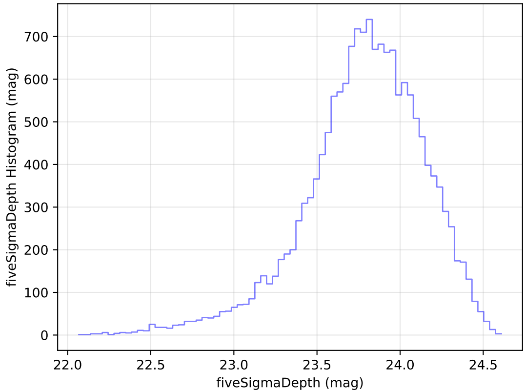
internal_u_expt60_nscale0.9v3.4_10yrs Yr 1 u band: fiveSigmaDepth Histogram
