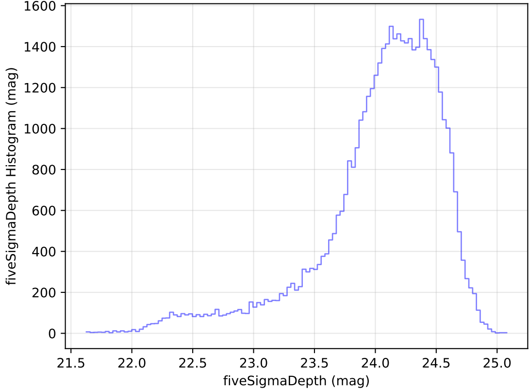
internal_u_expt60_nscale0.9v3.4_10yrs Yr 1 r band: fiveSigmaDepth Histogram
