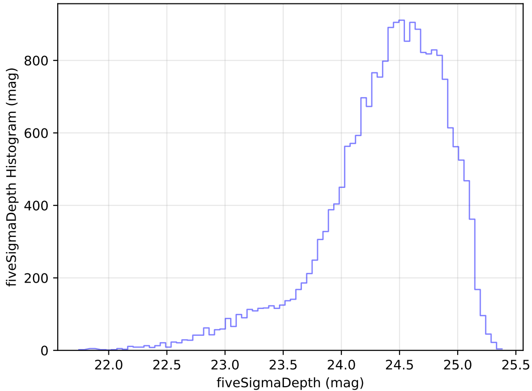
internal_u_expt60_nscale0.9v3.4_10yrs Yr 1 g band: fiveSigmaDepth Histogram
