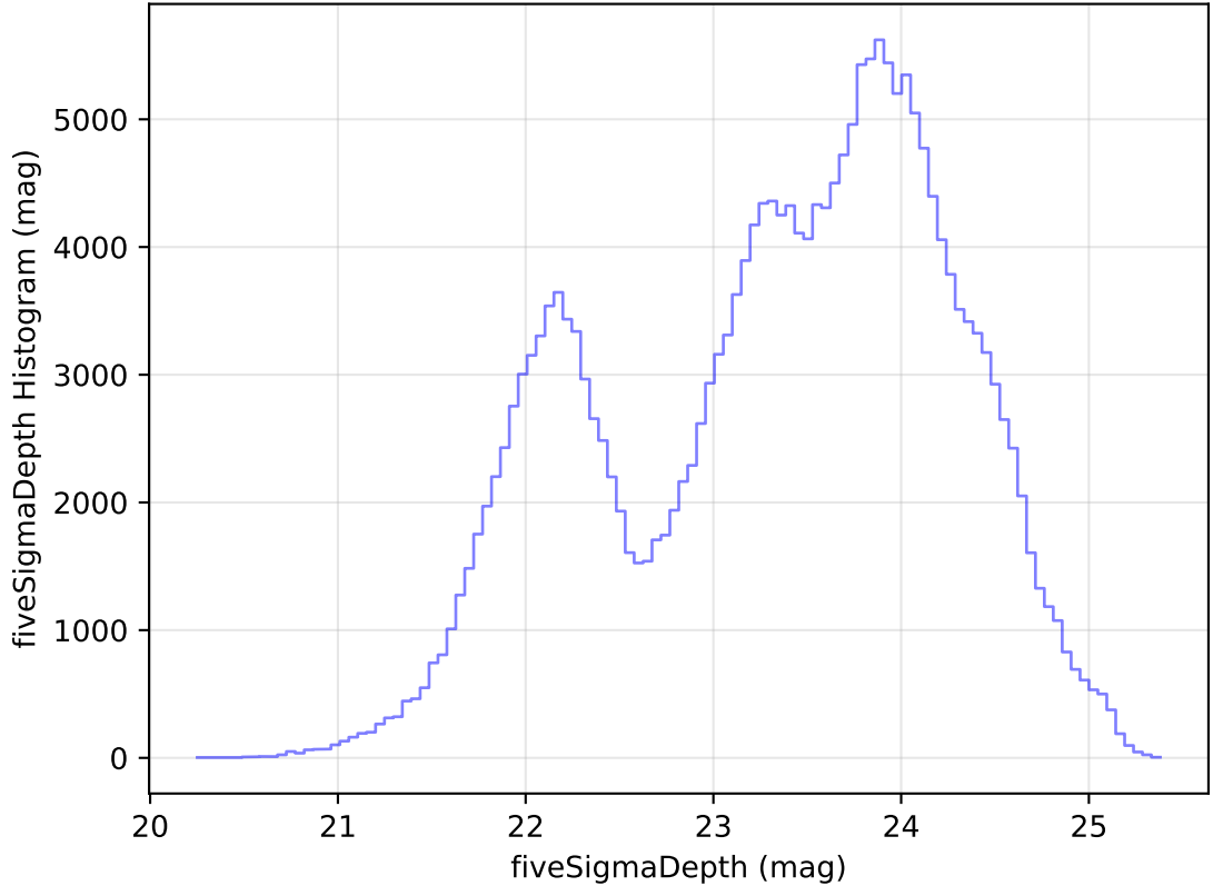
internal_u_expt60_nscale0.9v3.4_10yrs Yr 1 all bands: fiveSigmaDepth Histogram
