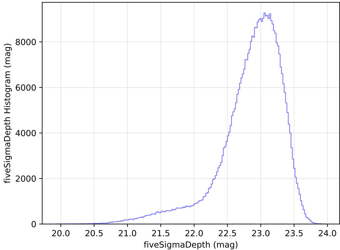
internal_u_expt60_nscale0.9v3.4_10yrs WFD z band: fiveSigmaDepth Histogram
