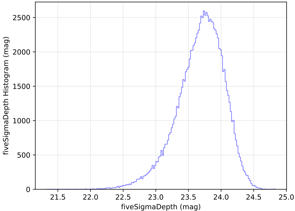
internal_u_expt60_nscale0.9v3.4_10yrs WFD u band: fiveSigmaDepth Histogram
