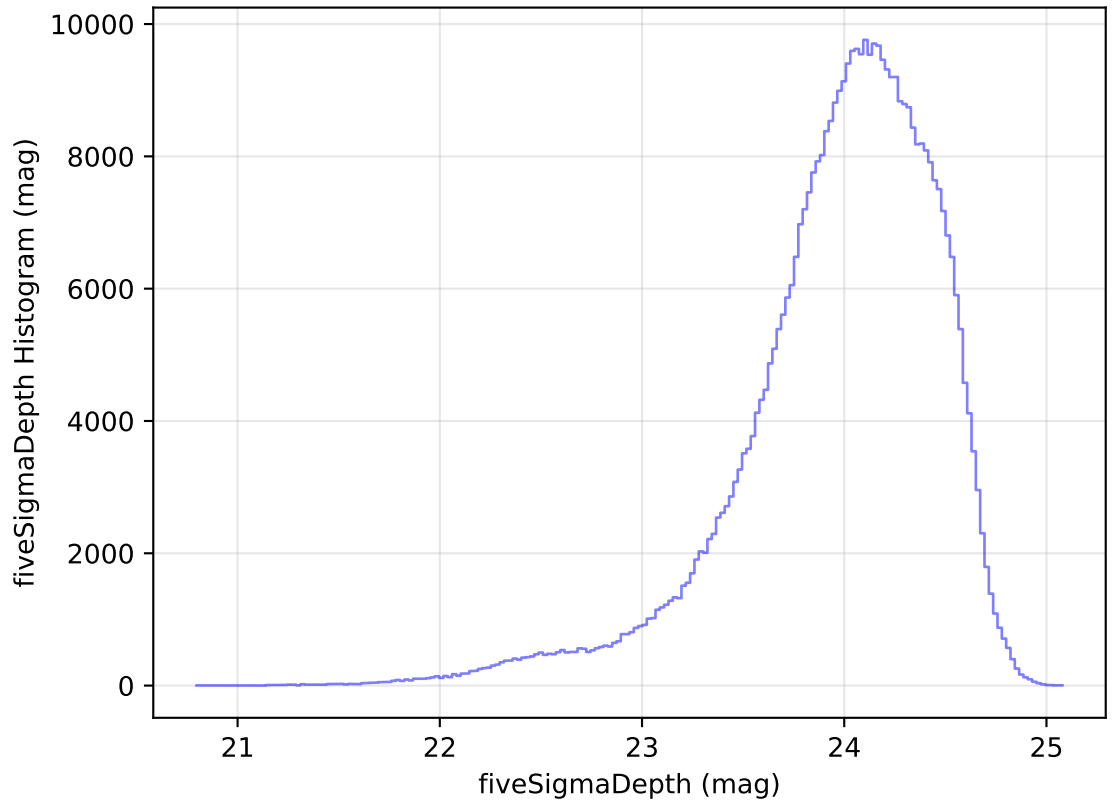
internal_u_expt60_nscale0.9v3.4_10yrs WFD r band: fiveSigmaDepth Histogram
