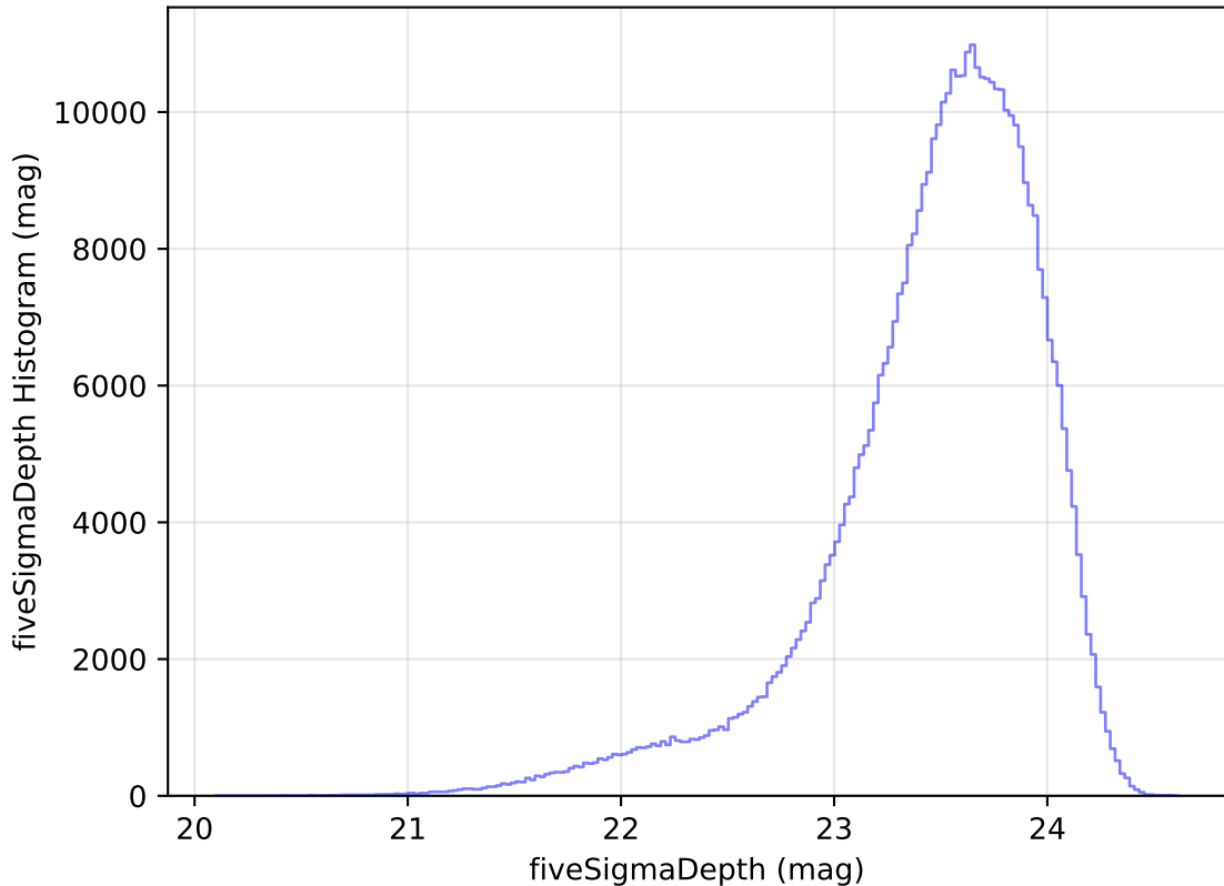
internal_u_expt60_nscale0.9v3.4_10yrs WFD i band: fiveSigmaDepth Histogram
