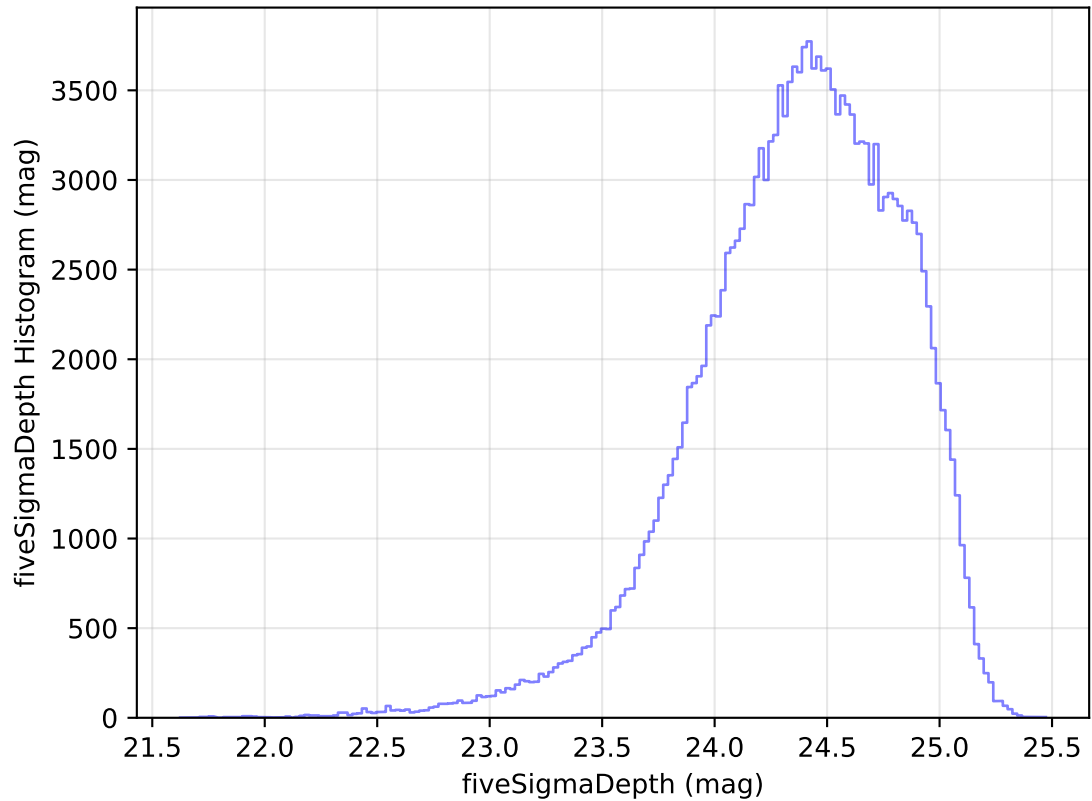
internal_u_expt60_nscale0.9v3.4_10yrs WFD g band: fiveSigmaDepth Histogram
