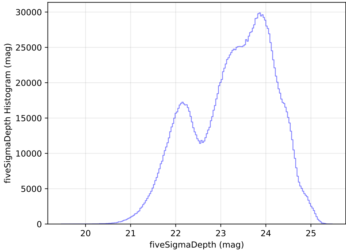
internal_u_expt60_nscale0.9v3.4_10yrs WFD all bands: fiveSigmaDepth Histogram
