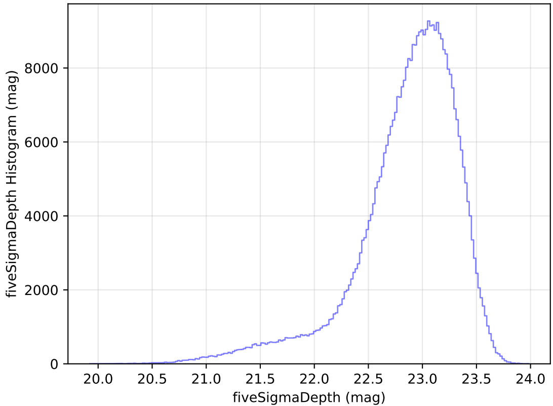
internal_u_expt60_nscale0.9v3.4_10yrs All sky z band: fiveSigmaDepth Histogram
