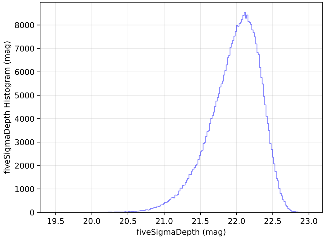
internal_u_expt60_nscale0.9v3.4_10yrs All sky y band: fiveSigmaDepth Histogram
