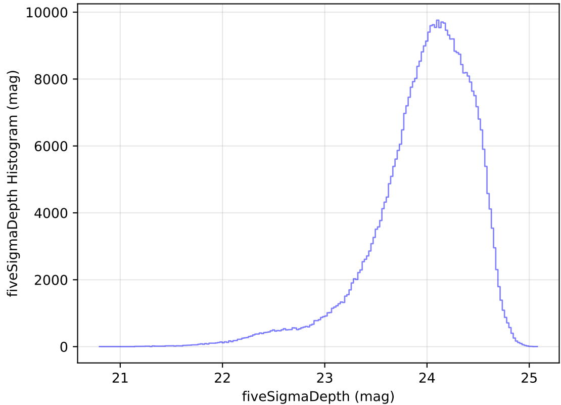
internal_u_expt60_nscale0.9v3.4_10yrs All sky r band: fiveSigmaDepth Histogram
