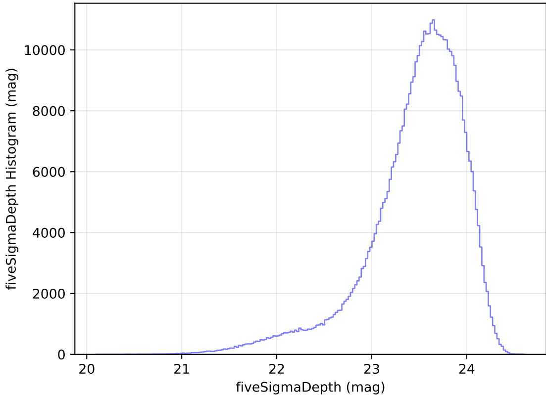
internal_u_expt60_nscale0.9v3.4_10yrs All sky i band: fiveSigmaDepth Histogram
