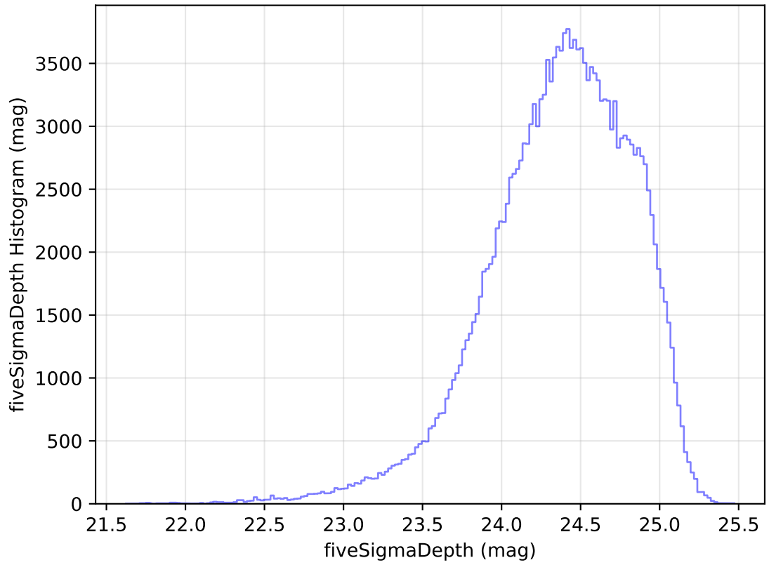
internal_u_expt60_nscale0.9v3.4_10yrs All sky g band: fiveSigmaDepth Histogram
