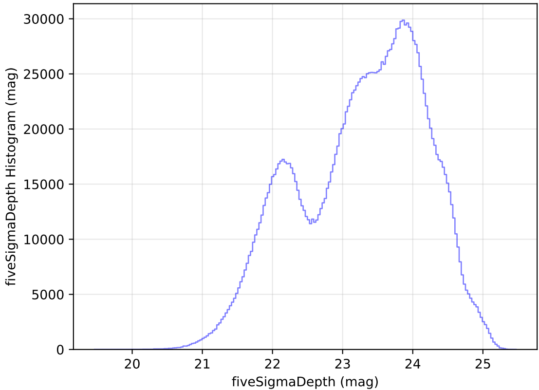
internal_u_expt60_nscale0.9v3.4_10yrs All sky all bands: fiveSigmaDepth Histogram
