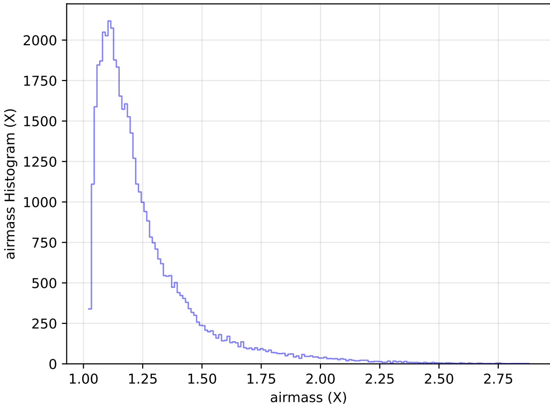
internal_u_expt60_nscale0.9v3.4_10yrs Yr 1 y band: airmass Histogram
