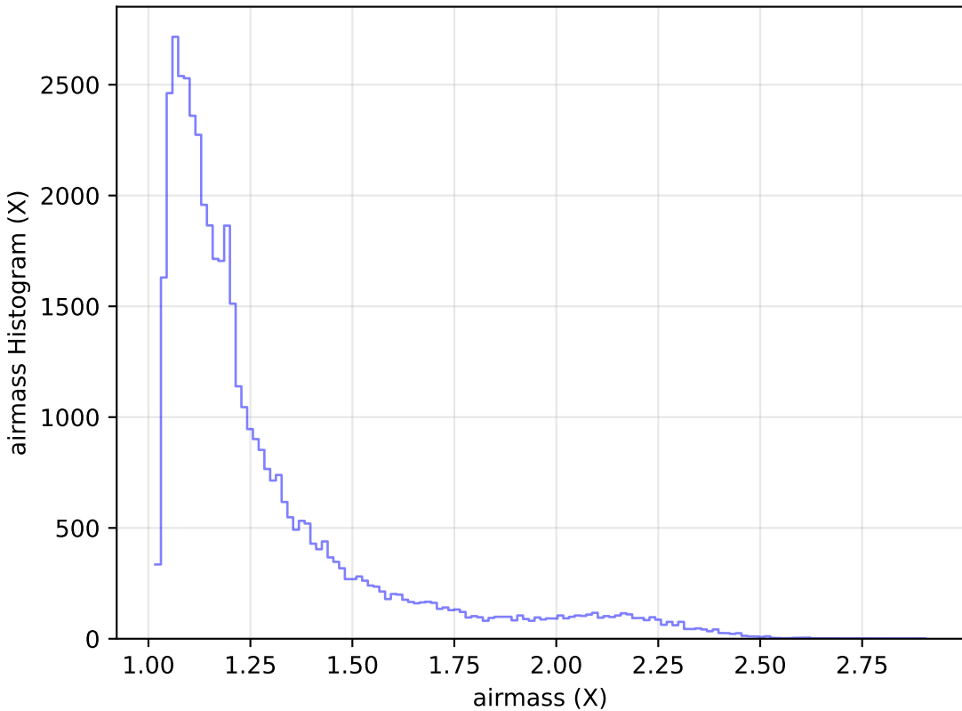
internal_u_expt60_nscale0.9v3.4_10yrs Yr 1 r band: airmass Histogram
