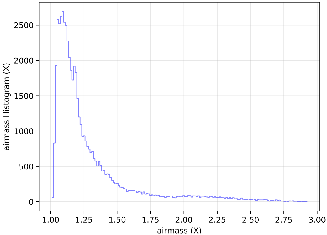
internal_u_expt60_nscale0.9v3.4_10yrs Yr 1 i band: airmass Histogram
