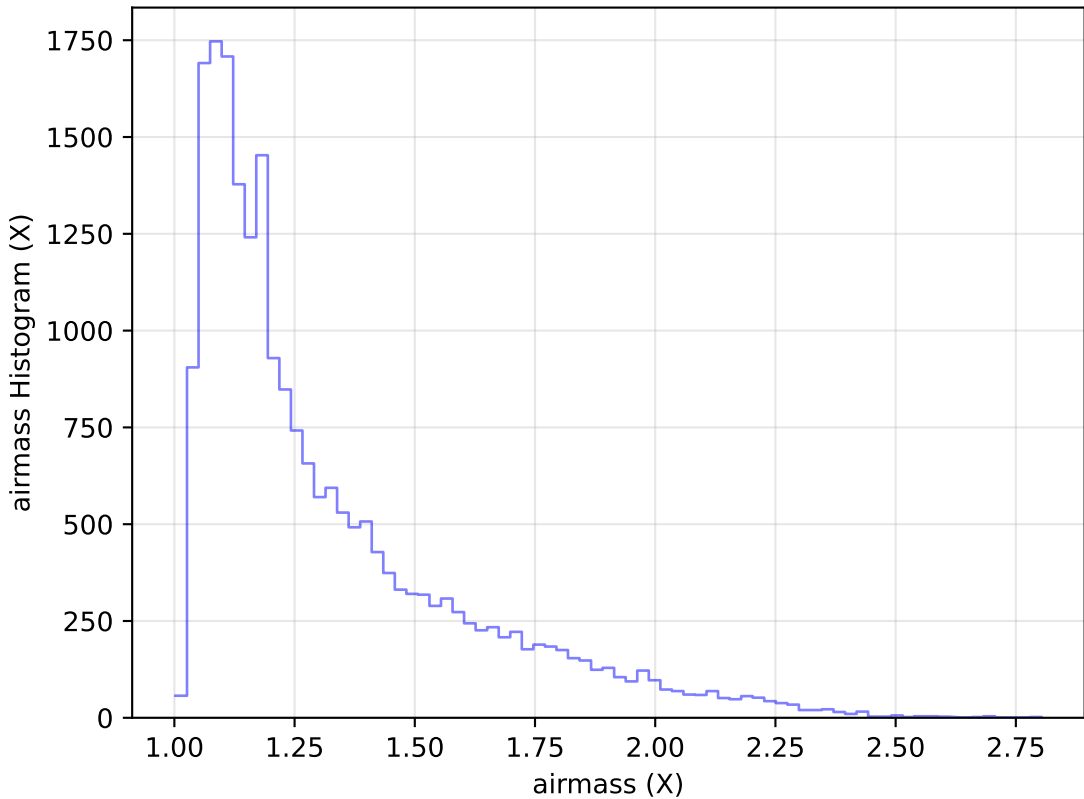
internal_u_expt60_nscale0.9v3.4_10yrs Yr 1 g band: airmass Histogram
