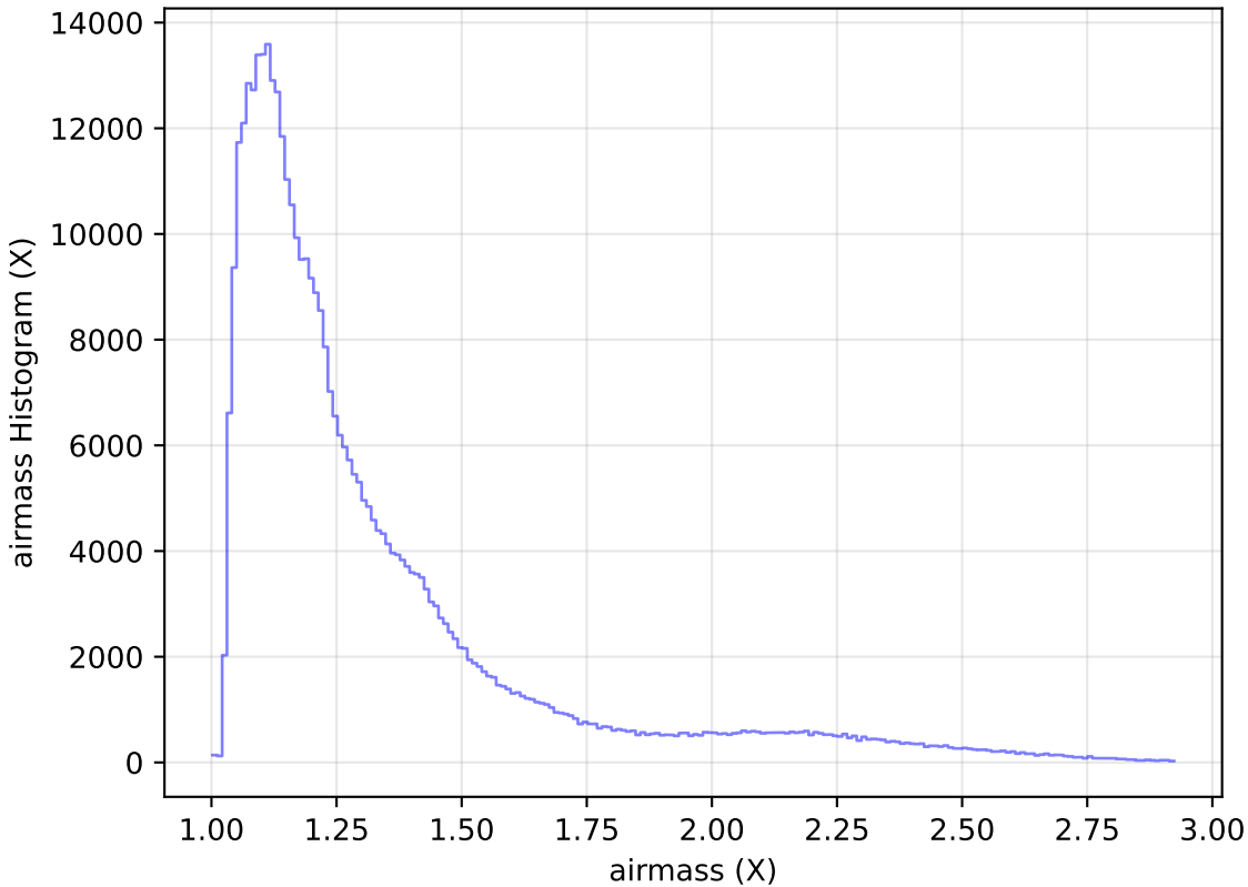
internal_u_expt60_nscale0.9v3.4_10yrs WFD z band: airmass Histogram
