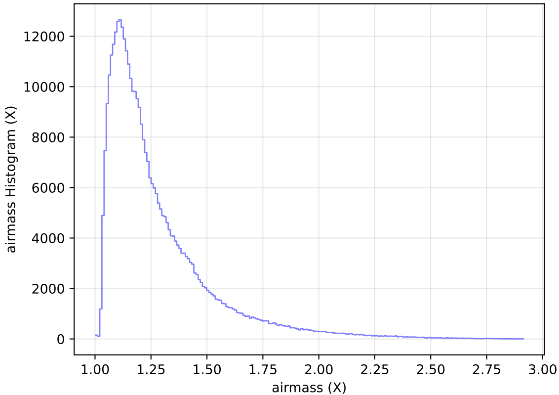
internal_u_expt60_nscale0.9v3.4_10yrs WFD y band: airmass Histogram
