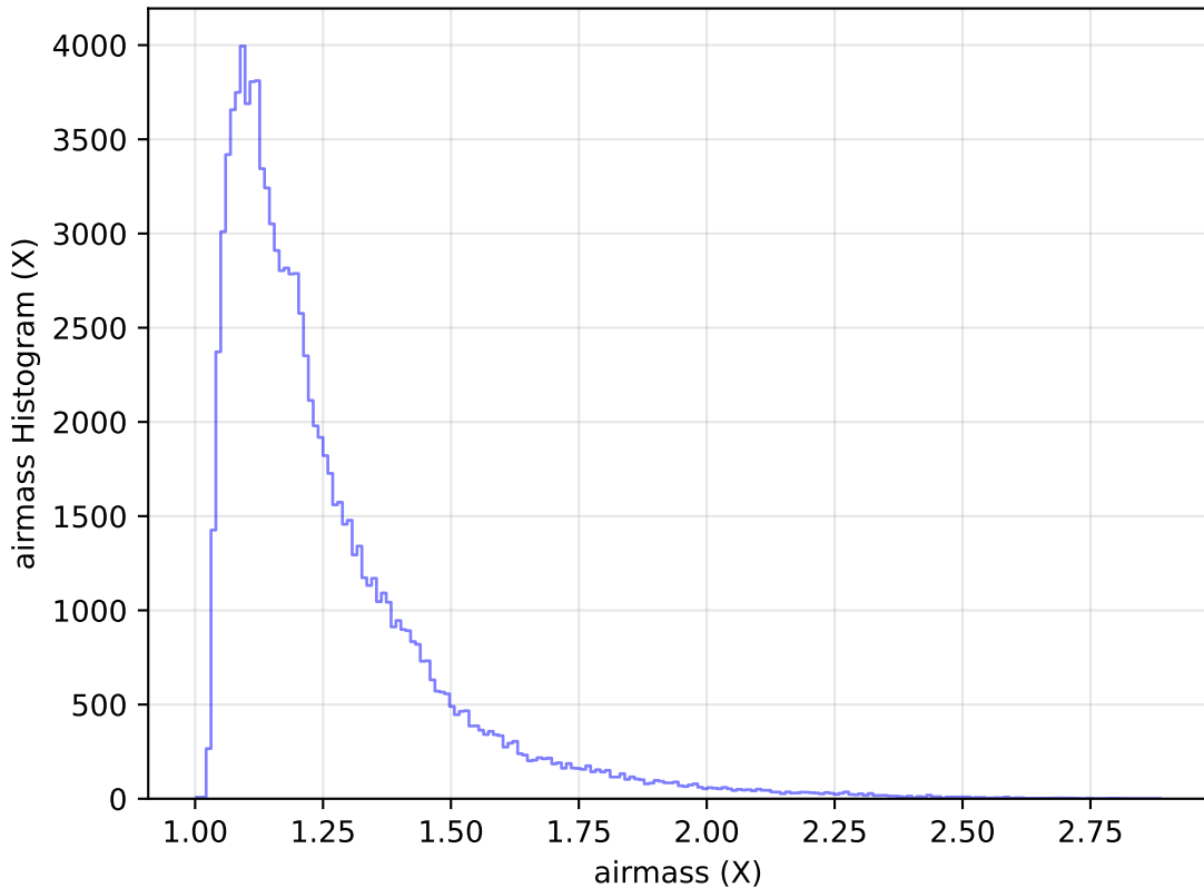
internal_u_expt60_nscale0.9v3.4_10yrs WFD u band: airmass Histogram
