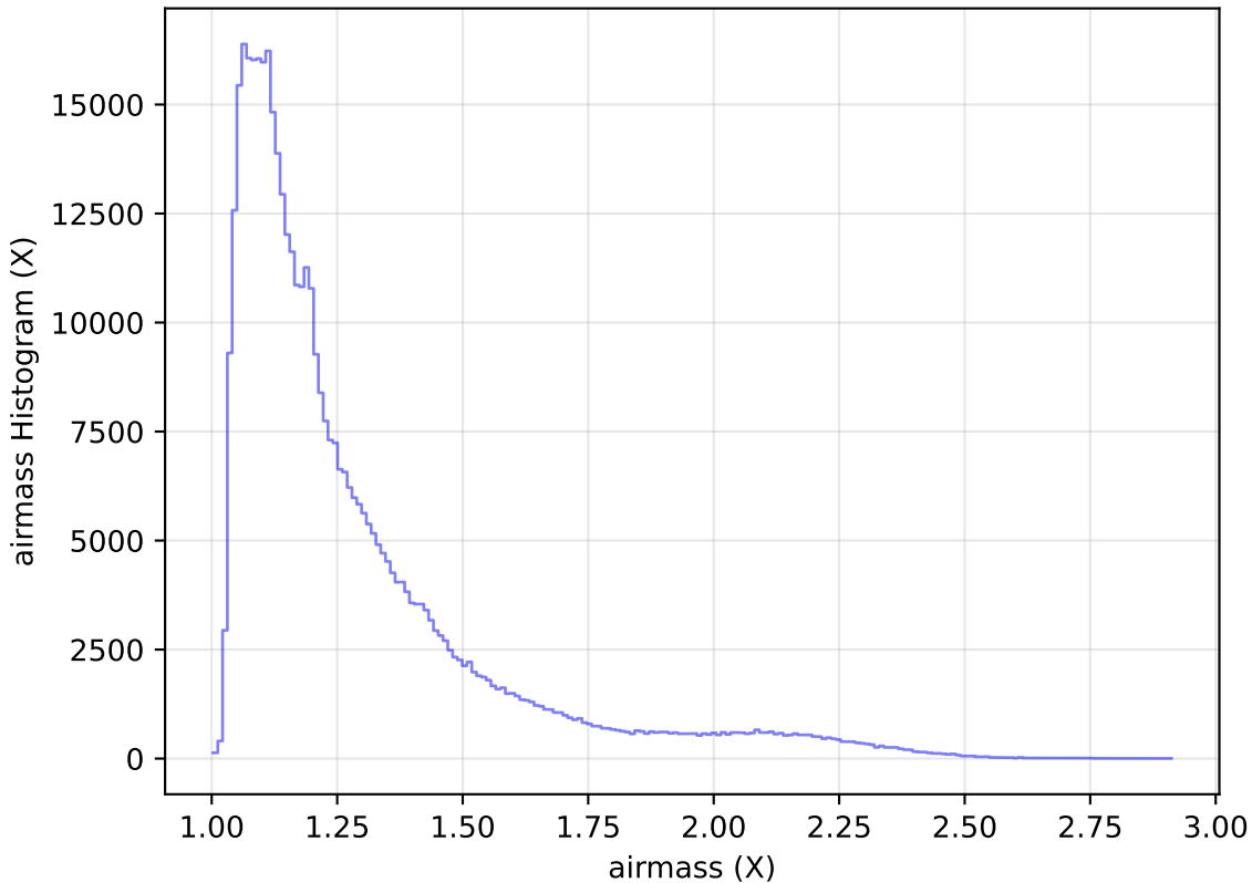
internal_u_expt60_nscale0.9v3.4_10yrs WFD r band: airmass Histogram
