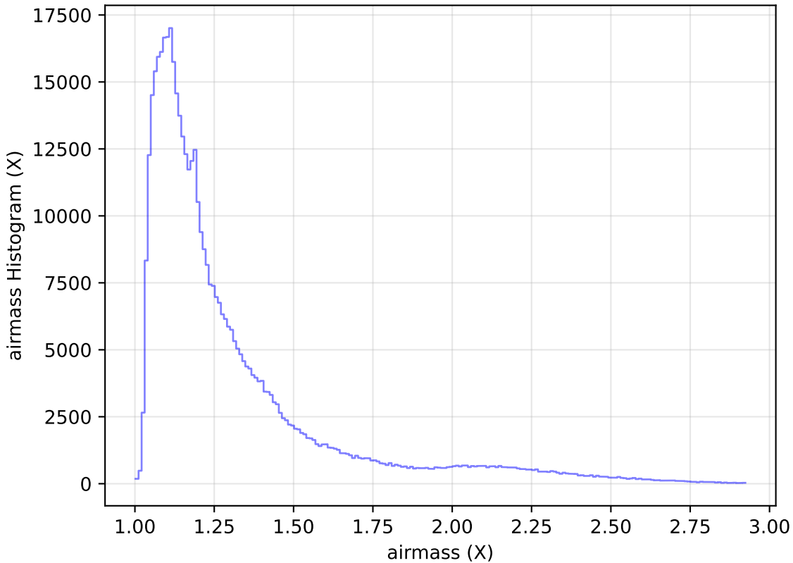
internal_u_expt60_nscale0.9v3.4_10yrs WFD i band: airmass Histogram
