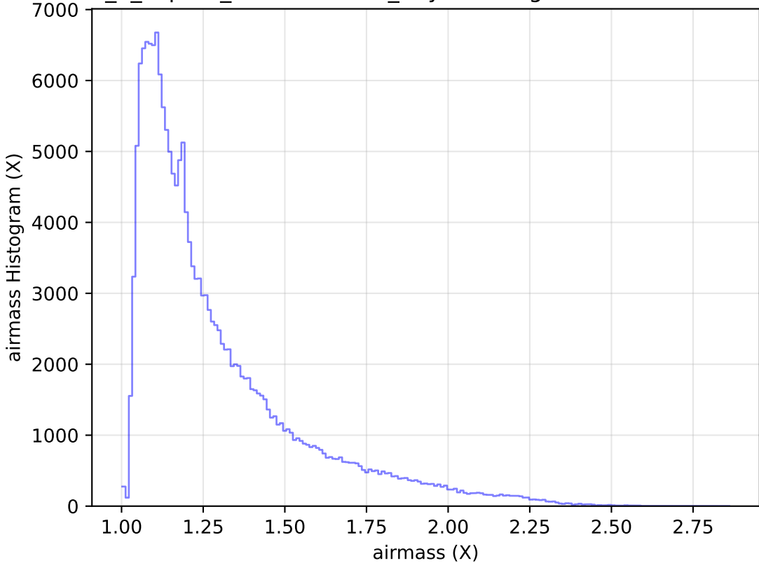
internal_u_expt60_nscale0.9v3.4_10yrs WFD g band: airmass Histogram
